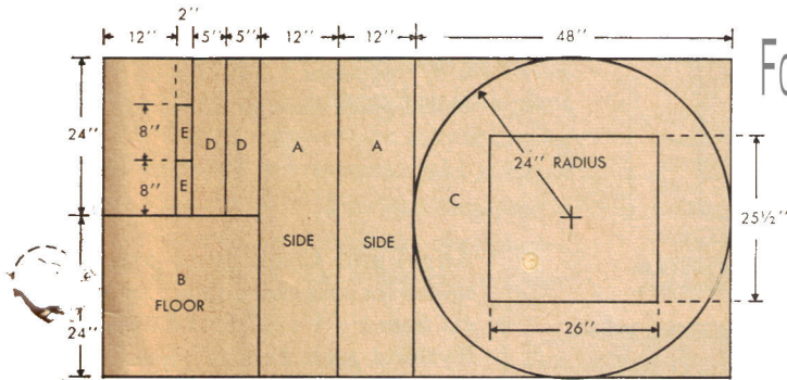
PLYWOOD CUTTING SCHEDULE
