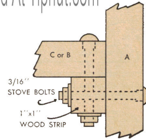
METHOD OF FASTENING FLOOR AND SEAT TO SIDES
